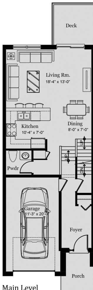
Main Level
